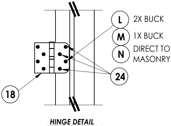
HINGE DETAIL
