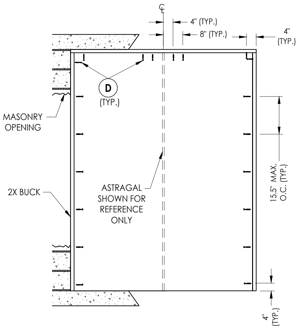
BUCK ANCHORING
