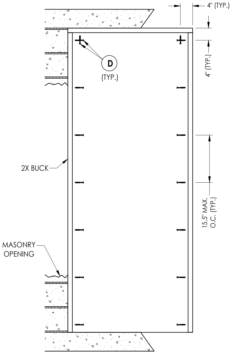
BUCK ANCHORING
